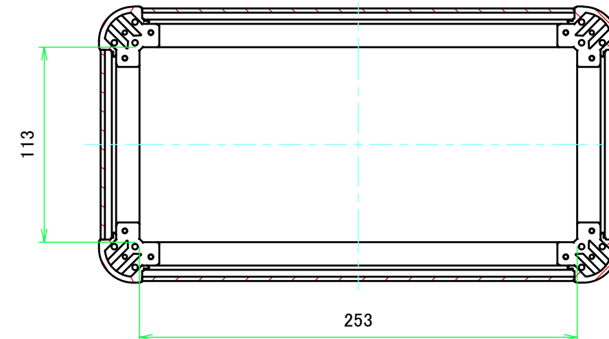
C-C (1:3)
